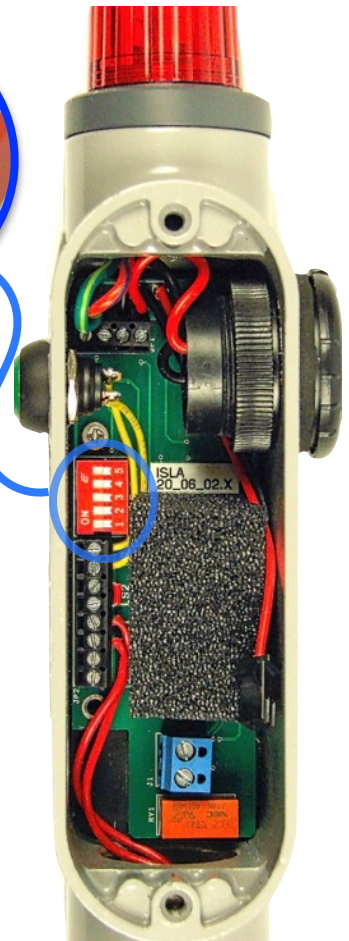
DIP SWITCH WITH #1 & 2 "ON"
